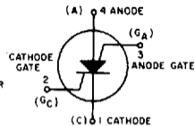
Thyristor Circuit
