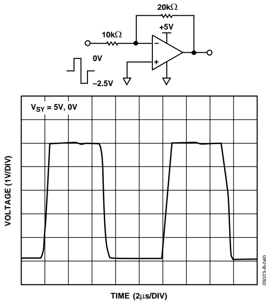
Figure 41. Gain of Two Inverter Response to 2.5 V Step, Centered -1.25 V below Ground
