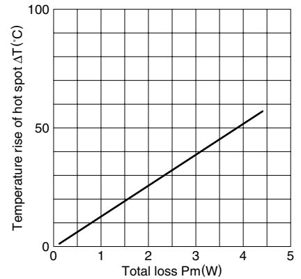
Temperature rise vs. Total loss for RM12 core (Typical) (Ambient temperature: 25°C)
