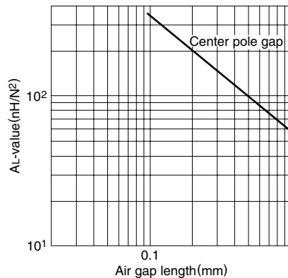
AL-value vs. Air gap length for PC50RM6 core (Typical)
