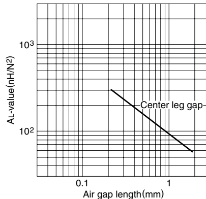
AL-value vs. Air gap length for PC40EE30/30/7 core (Typical)
