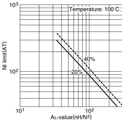
NI limit vs. AL-value for PC50RM6 gapped core (Typical)
