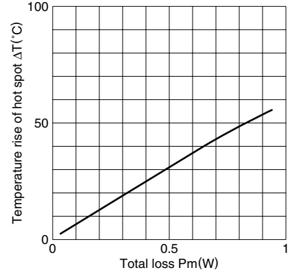
Temperature rise vs. Total loss for EE13 core (Typical) (Ambient temperature: 25°C)
