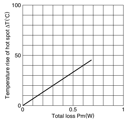
Temperature rise vs. Total loss for RM6 core (Typical) (Ambient temperature: 25°C)
