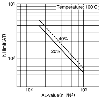
NI limit vs. AL-value for PC40EI40 gapped core (Typical)
