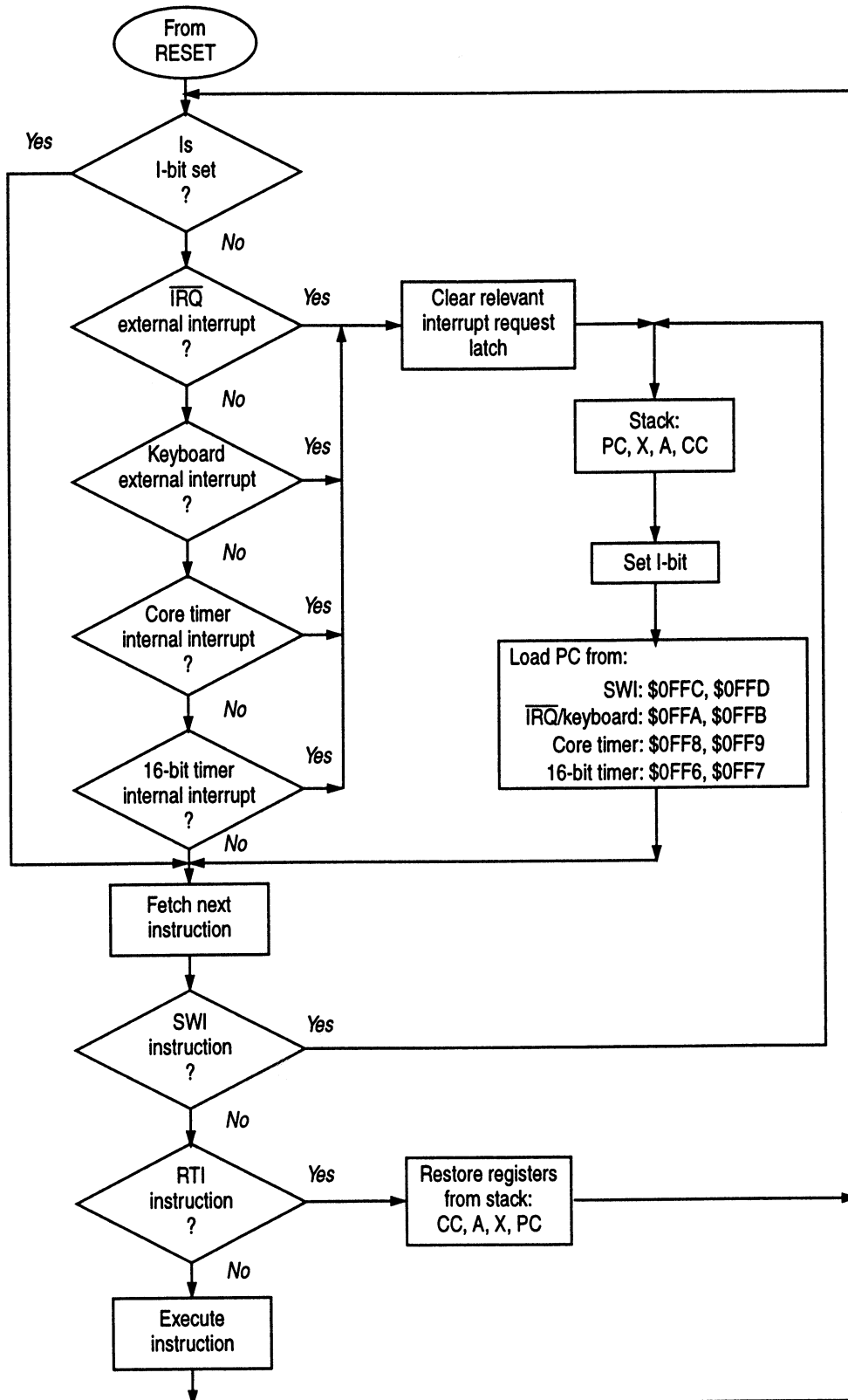
Figure 7-1 Interrupt flowchart
