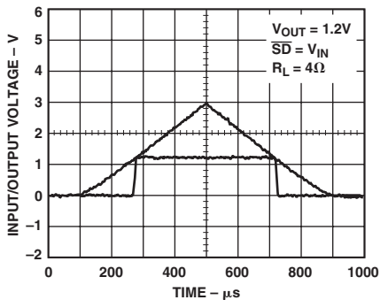
TPC 9. Power-Up/Power-Down
