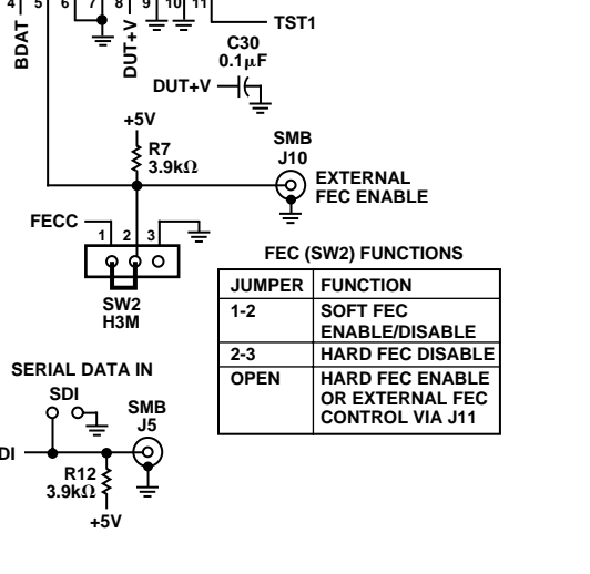
Figure 39. Electrical Schematic of AD9853-xxPCB Evaluation Board
