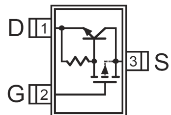
SOT-23 (Top View)
