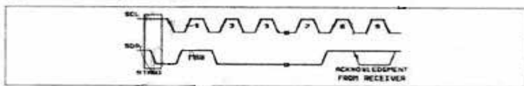
Figure 19: Acknowledge on the I 2 C BUS
