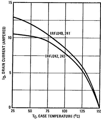
Fig. 13 - Maximum Drain Current Vs. Case Temperature
