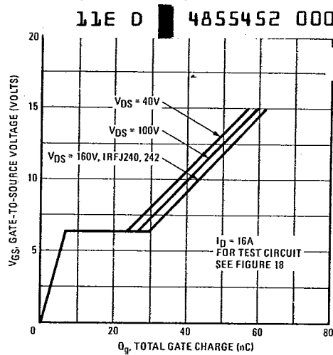
Fig. 11 - Typical Gate Charge Vs. Gate-to-Source Voltage
