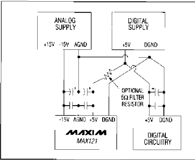
Figure 26. Power-Supply Grounding
