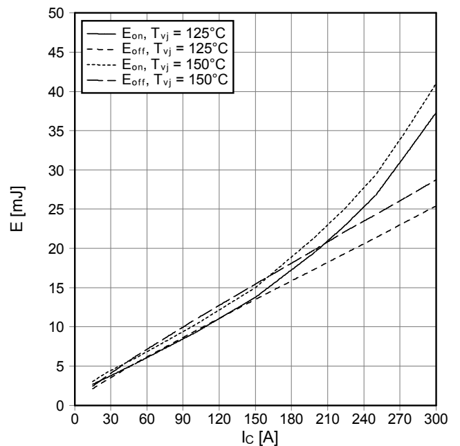
Schaltverluste IGBT-Brems-Chopper switching losses IGBT-brake-chopper E_{on} = f(I_c) , E_{off} = f(I_c) V_{GE} = \pm 15\text{ V} , R_{Gon} = 1.1\ \Omega , R_{Goff} = 1.1\ \Omega , V_{CE} = 600\text{ V}
