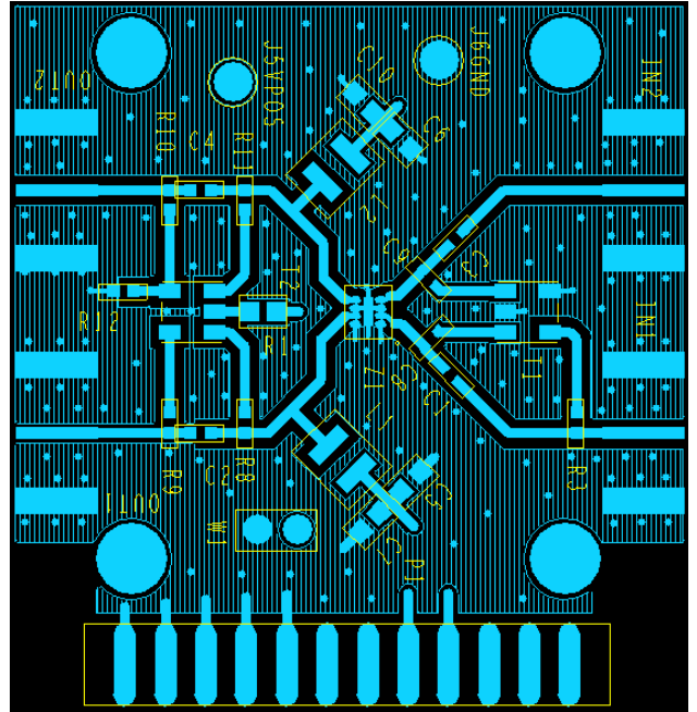
Figure 25. Evaluation Board Layout
