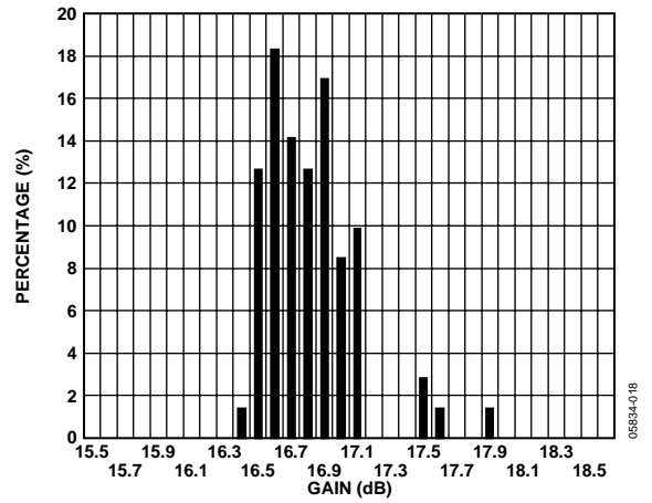
Figure 18. Gain Distribution at 190 MHz, VPOS = 5 V
