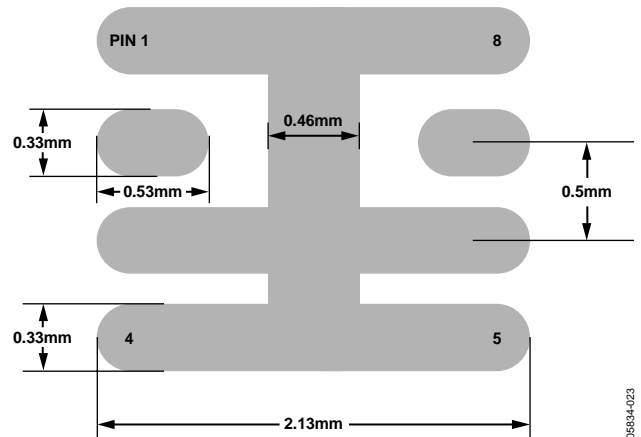
Figure 23. Recommended Land Pattern
