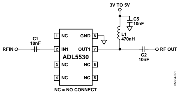
Figure 21. Basic Connections
