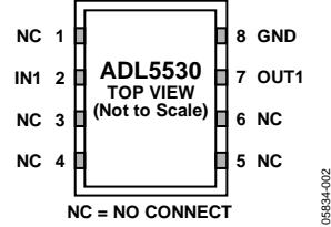
Figure 2. Pin Configuration
