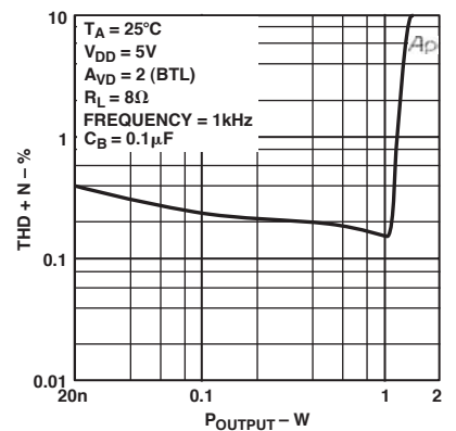
TPC 8. THD+N vs. P_{OUTPUT}
