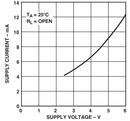
TPC 30. Supply Current vs. Supply Voltage
