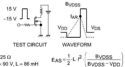
Fig. 8.16 Test Circuit/Waveform
