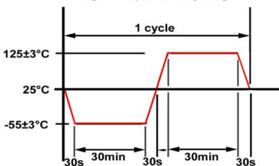
Fig 1 Temperature cycling
