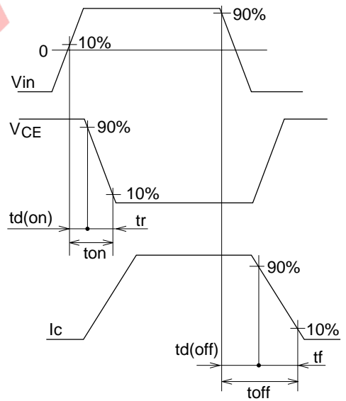
Waveform
