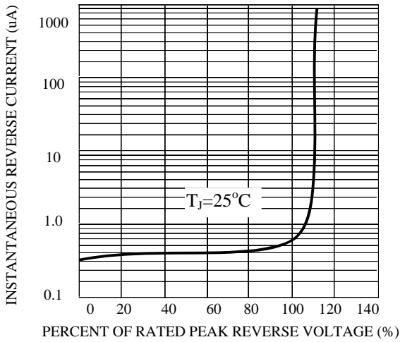
FIG. 3-TYPICAL REVERSE CHARACTERISTICS
