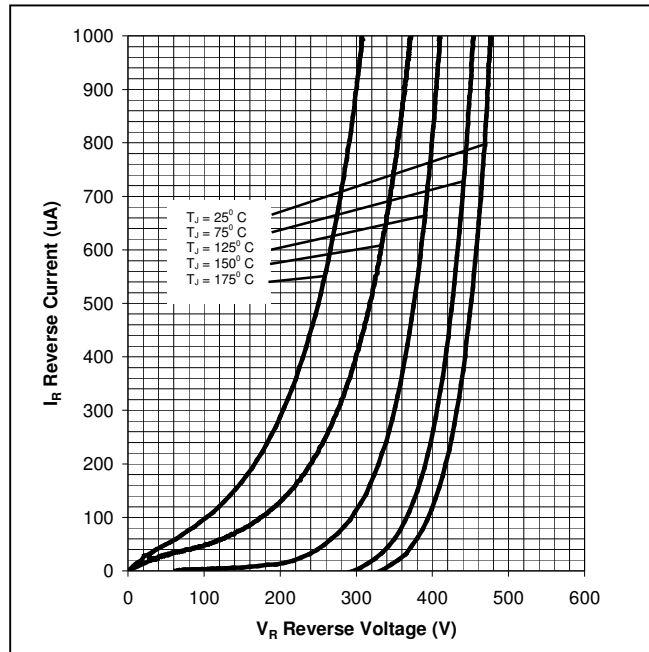
Figure 2. Reverse Characteristics
