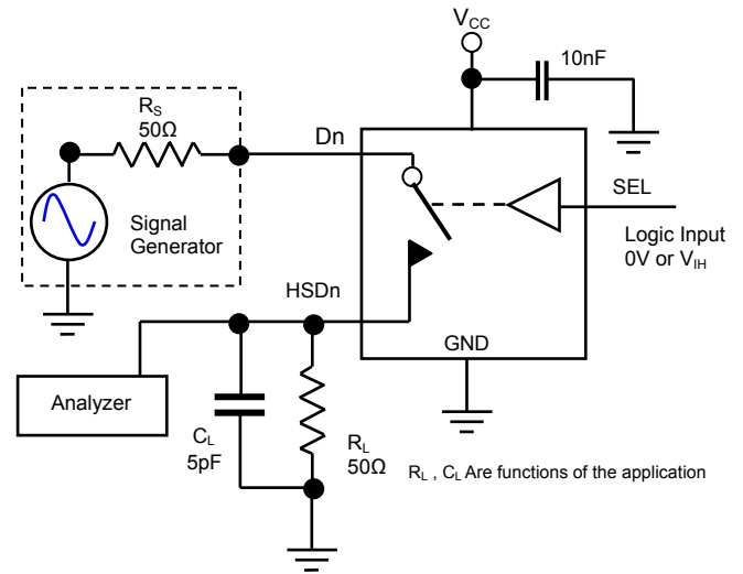
Fig.9 Channel Off Isolation
