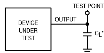
Figure 2. Test Circuit
