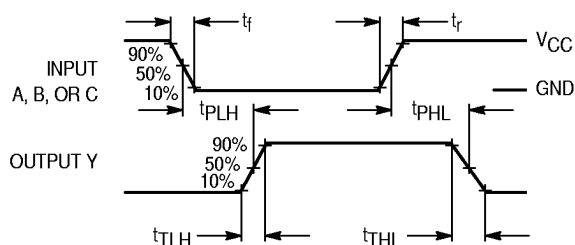
Figure 1. Switching Waveforms
