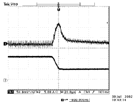
Vout=3.3V 100% to 50% load transients at 5V input and Ta=25° C
