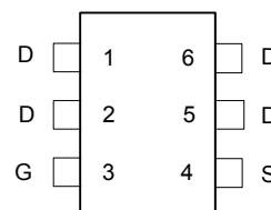
Top View of SOT-23-6
