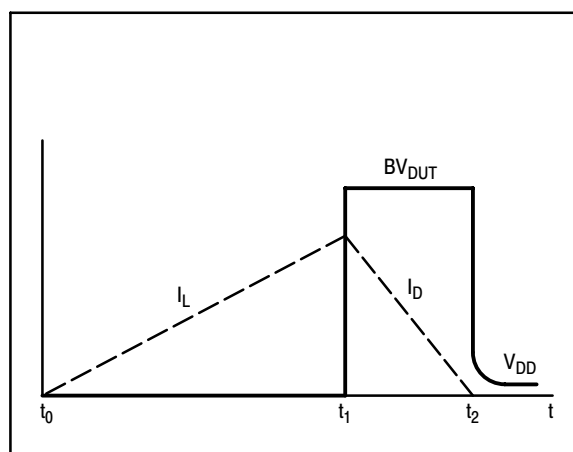
Figure 10. Current-Voltage Waveforms
