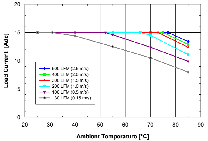
Fig. 10: Available load current vs. ambient air temperature and airflow rates for ASQ48T15033 converter with D height pins mounted horizontally with V_{in} = 48\text{ V} , air flowing from pin 3 to pin 1 and maximum FET temperature \leq 120^{\circ}\text{C} .
