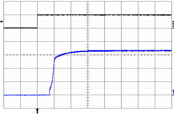
Fig. 17: Turn-on transient at full rated load current (resistive) with no output capacitor at V_{in} = 48\text{ V} , triggered via ON/OFF pin. Top trace: ON/OFF signal (5 V/div.). Bottom trace: output voltage (1 V/div.) Time scale: 2 ms/div.
