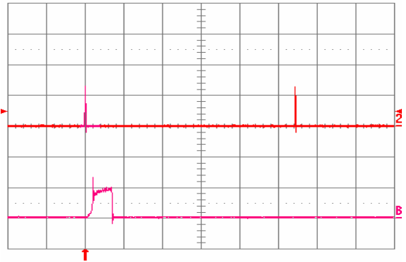
Fig. 26: Load current (top trace, 20 A/div, 20 ms/div) into a 10 mΩ short circuit during restart, at V_{in} = 48 V. Bottom trace (20 A/div, 1 ms/div) is an expansion of the on-time portion of the top trace.
