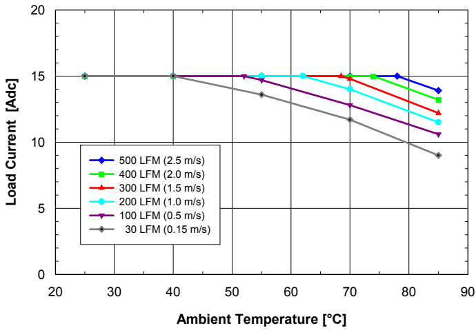
Fig. 9: Available load current vs. ambient air temperature and airflow rates for ASQ48T15033 converter with D height pins mounted vertically with V_{in} = 48\text{ V} , air flowing from pin 3 to pin 1 and maximum FET temperature \leq 120^{\circ}\text{C} .
