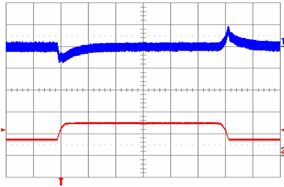
Fig. 19: Output voltage response to load current step-change (3.75 A – 7.5 A – 3.75 A) at V_{in} = 48\text{ V} . Top trace: output voltage (100 mV/div). Bottom trace: load current (5 A/div.). Current slew rate: 0.1 A/ \mu\text{s} . C_o = 1\ \mu\text{F} ceramic. Time scale: 0.2 ms/div.
