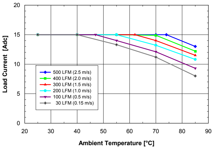
Fig. 11: Available load current vs. ambient temperature and airflow rates for ASQ48S15033 converter mounted vertically with V_{in} = 48\text{ V} , air flowing from pin 3 to pin 1 and maximum FET temperature \leq 120^{\circ}\text{C} .
