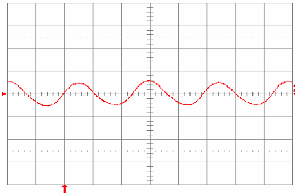
Fig. 23: Input reflected ripple current, i_c (100 mA/div), measured at input terminals at full rated load current and V_{in} = 48 \text{ V} . Refer to Fig. 22 for test setup. Time scale: 1 \mu\text{s}/\text{div} .
