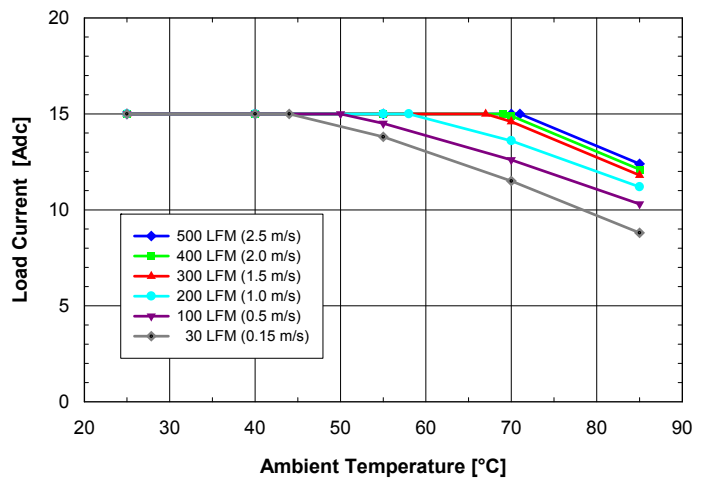
Fig. 12: Available load current vs. ambient temperature and airflow rates for ASQ48S15033 converter mounted horizontally with V_{in} = 48\text{ V} , air flowing from pin 3 to pin 1 and maximum FET temperature \leq 120^{\circ}\text{C} .
