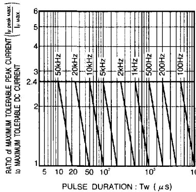
Fig. 7 Maximum tolerable peak current vs. pulse duration (green)
