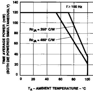
Figure 6a. Maximum Allowable Average Power vs. Ambient Temperature, HLMA-VL00/VH00.
