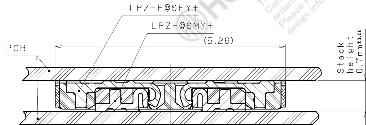
△ Mating detail (Reference)
