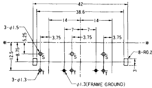
HOLE LAYOUT (PRINTED-SIDE VIEW) PWB t=1.6
