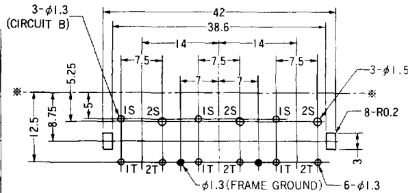
HOLE LAYOUT (PRINTED-SIDE VIEW) PWB t=1.6
