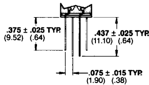
DIP SOLDER CODE Z
