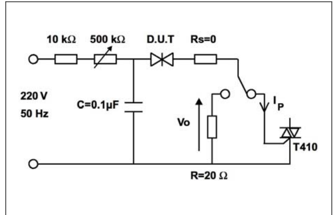
Diagram 2. Test circuit
