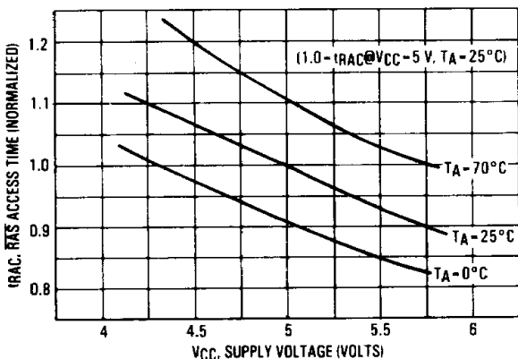
FIGURE 2 — \overline{RAS} ACCESS TIME versus SUPPLY VOLTAGE
