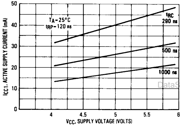
FIGURE 10 - I_{CC1} SUPPLY CURRENT versus SUPPLY VOLTAGE
