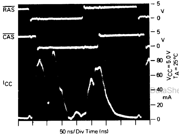
FIGURE 20 — \overline{\text{RAS}}/\overline{\text{CAS}} CYCLE
