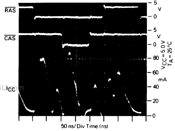
FIGURE 21 — LONG \overline{\text{RAS}}/\overline{\text{CAS}} CYCLE
