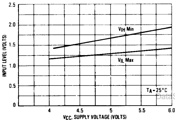
FIGURE 16 – ADDRESS INPUT LEVEL versus SUPPLY VOLTAGE
