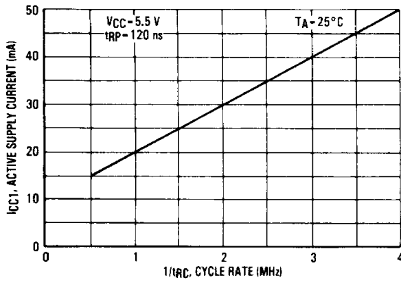
FIGURE 8 - I_{CC1} SUPPLY CURRENT versus CYCLE RATE
