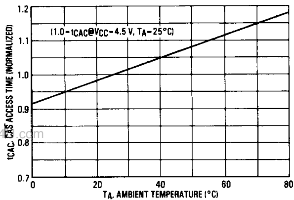
FIGURE 5 — \overline{CAS} ACCESS TIME versus AMBIENT TEMPERATURE
