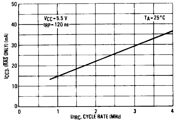
FIGURE 15 – I_{CC3} SUPPLY CURRENT versus CYCLE RATE
