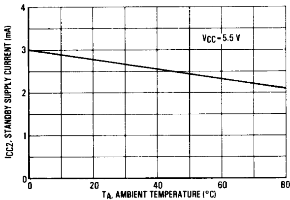
FIGURE 14 – I_{CC2} STANDBY CURRENT versus AMBIENT TEMPERATURE
