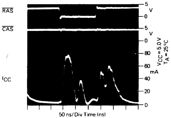
FIGURE 22 — \overline{\text{RAS}} ONLY CYCLE
