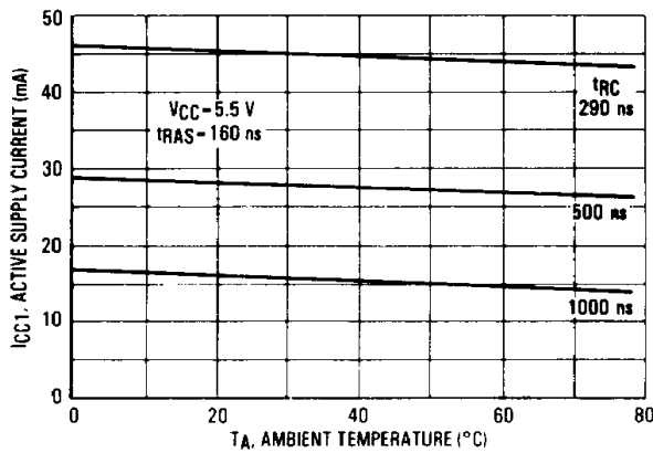
FIGURE 12 - I_{CC1} SUPPLY CURRENT versus AMBIENT TEMPERATURE (min t RAS )
