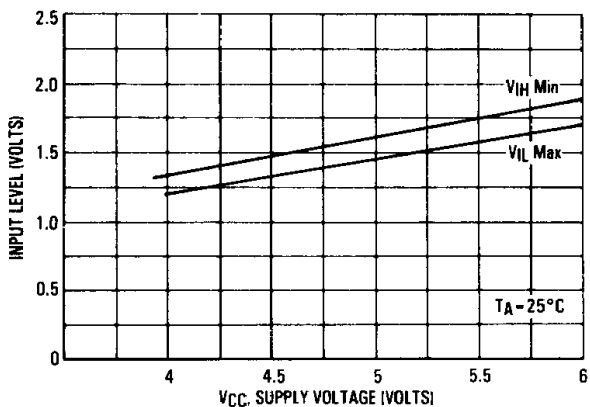
FIGURE 6 — \overline{RAS}, \overline{W} INPUT LEVEL versus SUPPLY VOLTAGE
