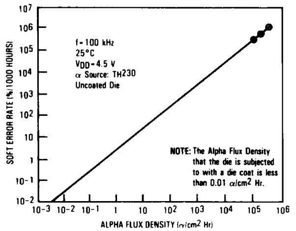
FIGURE 19 — SOFT ERROR RATE versus ALPHA FLUX DENSITY
