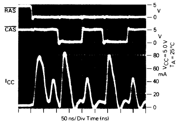
FIGURE 23 — PAGE MODE CYCLE
