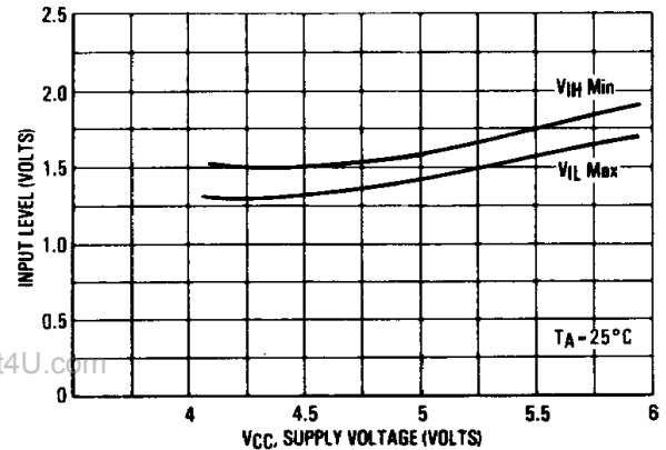
FIGURE 17 – DATA INPUT LEVEL versus SUPPLY VOLTAGE
