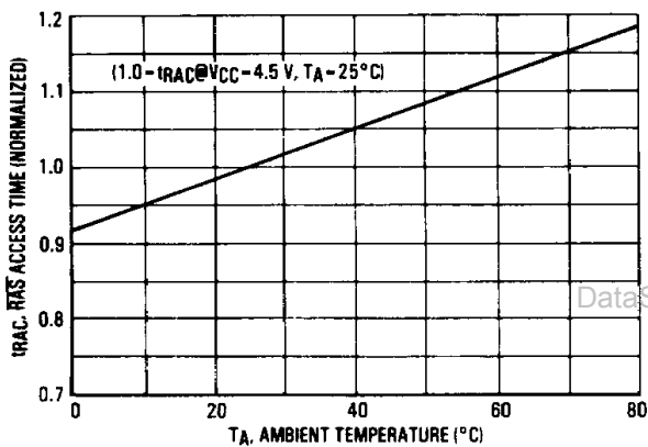
FIGURE 4 — \overline{RAS} ACCESS TIME versus AMBIENT TEMPERATURE
