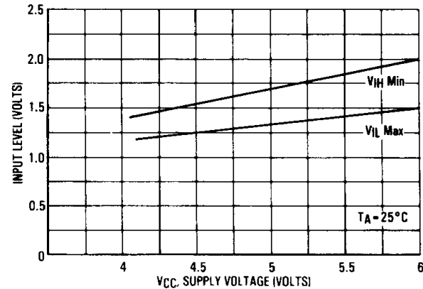
FIGURE 7 — \overline{CAS}, \overline{W} INPUT LEVEL versus SUPPLY VOLTAGE
