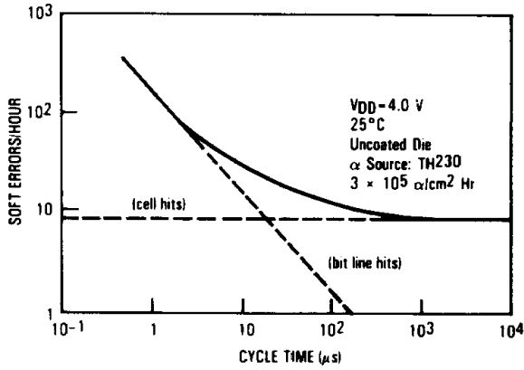
FIGURE 18 — ACCELERATED SOFT ERROR versus CYCLE TIME
