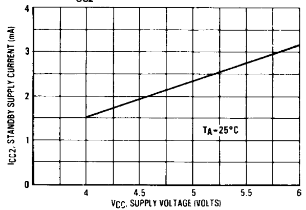
FIGURE 13 - I_{CC2} SUPPLY CURRENT versus SUPPLY VOLTAGE
