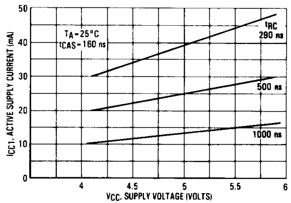
FIGURE 9 - I_{CC1} SUPPLY CURRENT versus SUPPLY VOLTAGE
