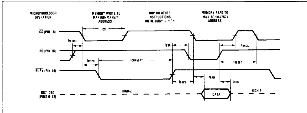
Figure 5. Static RAM Mode Timing Diagram
