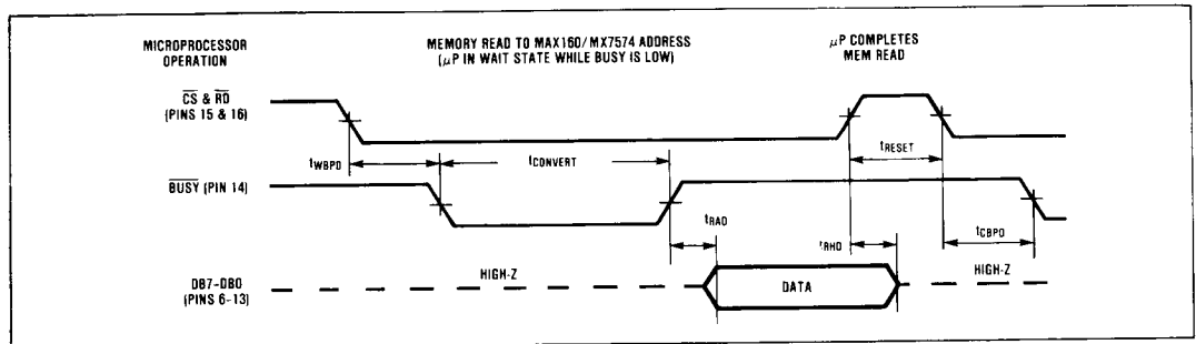
Figure 7. Slow Memory Mode Timing Diagram ( \overline{CS} and \overline{RD} Tied Together)
