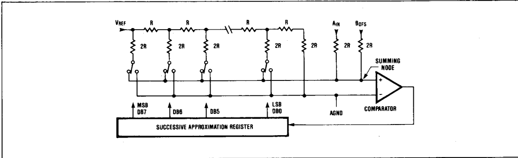
Figure 4. D/A Converter Used in the MAX160/MX7574
