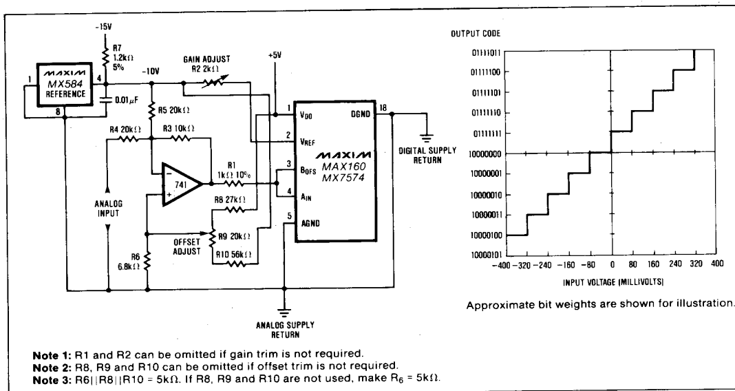
Figure 12. Bipolar (-10V to +10V) Operation and Nominal Transfer Characteristic Around Major Carry (Output Code is Complimentary Offset Binary)
