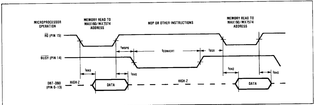
Figure 6. ROM Mode Timing Diagram ( \overline{CS} Held Low)
