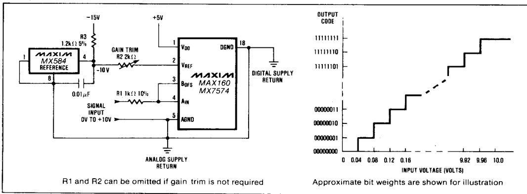
Figure 10. Unipolar (0V to +10V) Operation and Nominal Transfer Characteristic (Output Code is Straight Binary)
