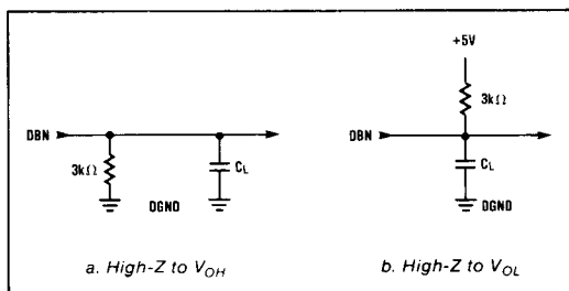
Figure 1. Load Circuits for Data Access Time Test
