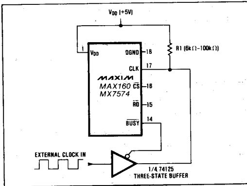
Figure 9. External Clock Operation (Static RAM and Slow Memory Mode)
