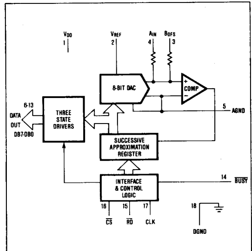
Figure 3. MAX160/MX7574 Functional Diagram
