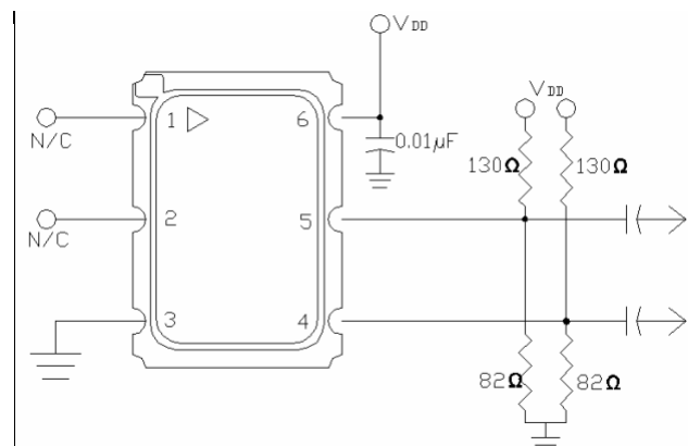
Figure 7. Pull-up Pull-down Termination
