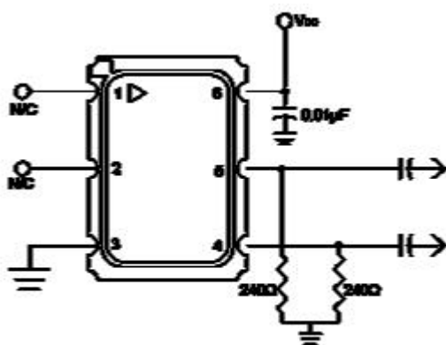
Figure 6. Single Resistor Termination
