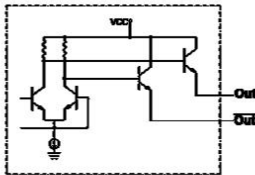
Figure 5. Standard PECL Output Configuration
