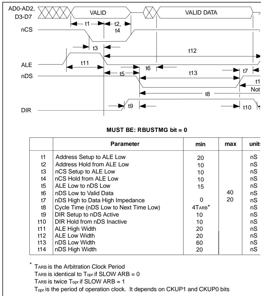
FIGURE 11 - MULTIPLEXED BUS, 68XX-LIKE CONTROL SIGNALS; READ CYCLE
