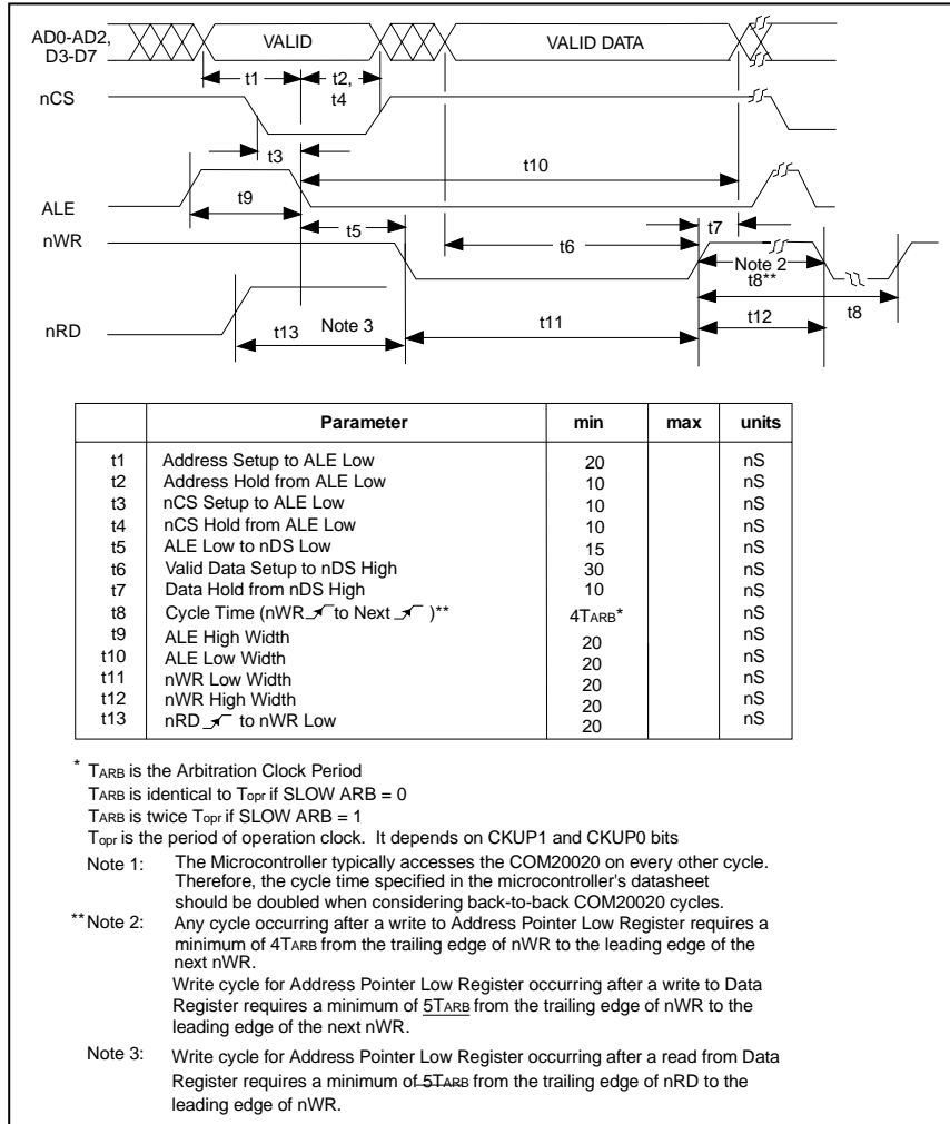
FIGURE 14 - MULTIPLEXED BUS, 80XX-LIKE CONTROL SIGNALS; WRITE CYCLE
