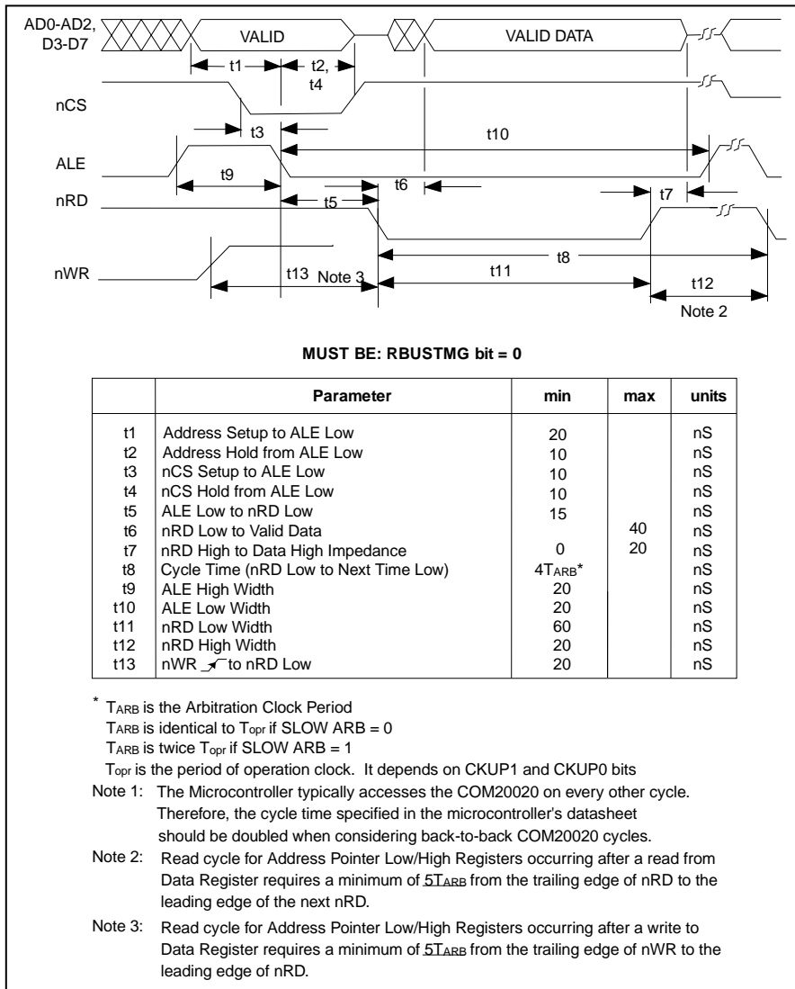
FIGURE 12 - MULTIPLEXED BUS, 80XX-LIKE CONTROL SIGNALS; READ CYCLE
