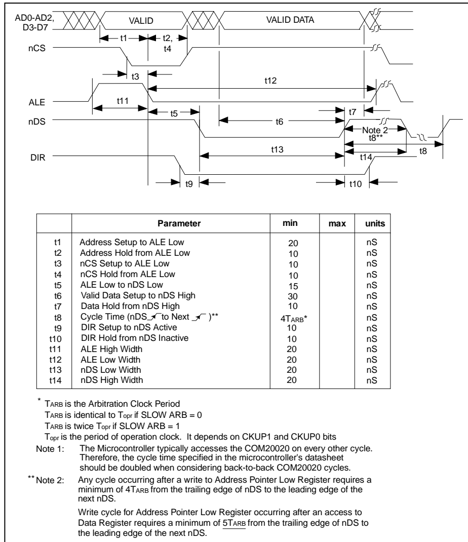
FIGURE 13 - MULTIPLEXED BUS, 68XX-LIKE CONTROL SIGNALS; WRITE CYCLE
