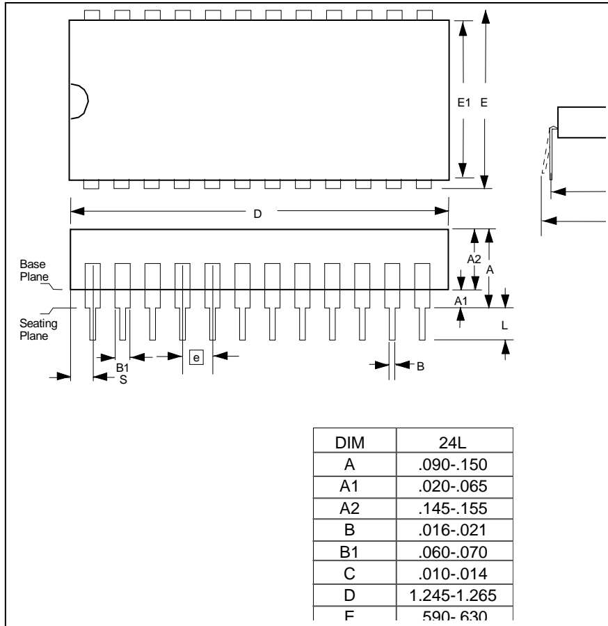
FIGURE 24 - 24 PIN DIP PACKAGE DIMENSIONS
