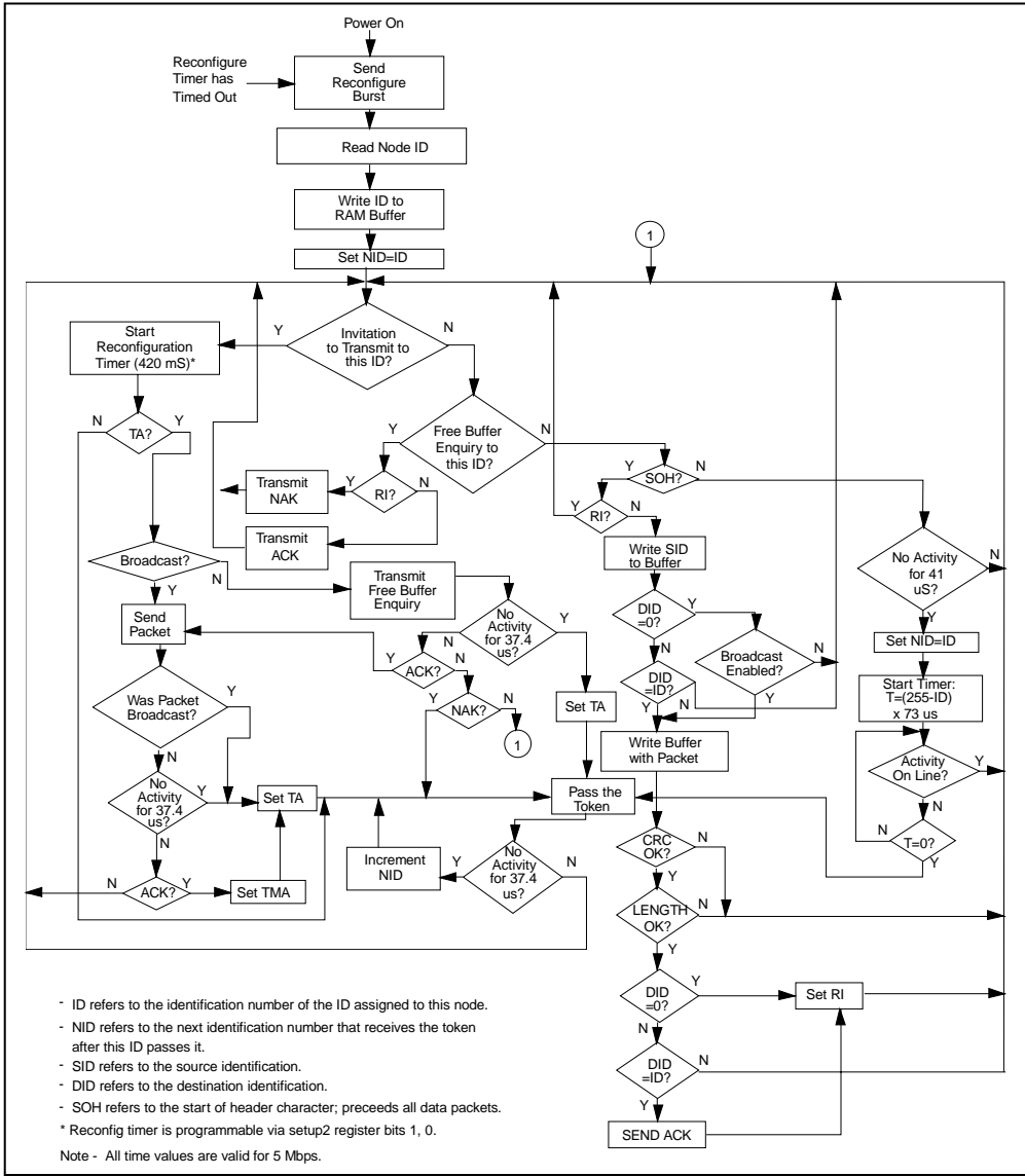
FIGURE 1 - COM20020 OPERATION
