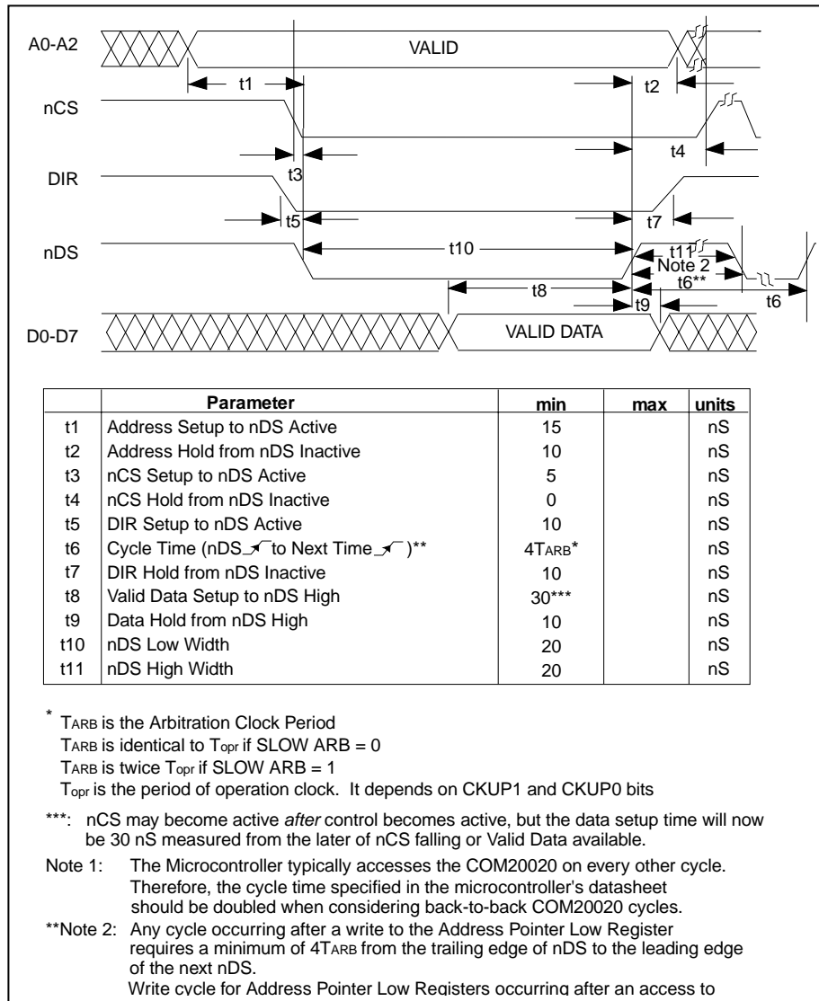
FIGURE 18 - NON-MULTIPLEXED BUS, 68XX-LIKE CONTROL SIGNALS; WRITE CYCLE
