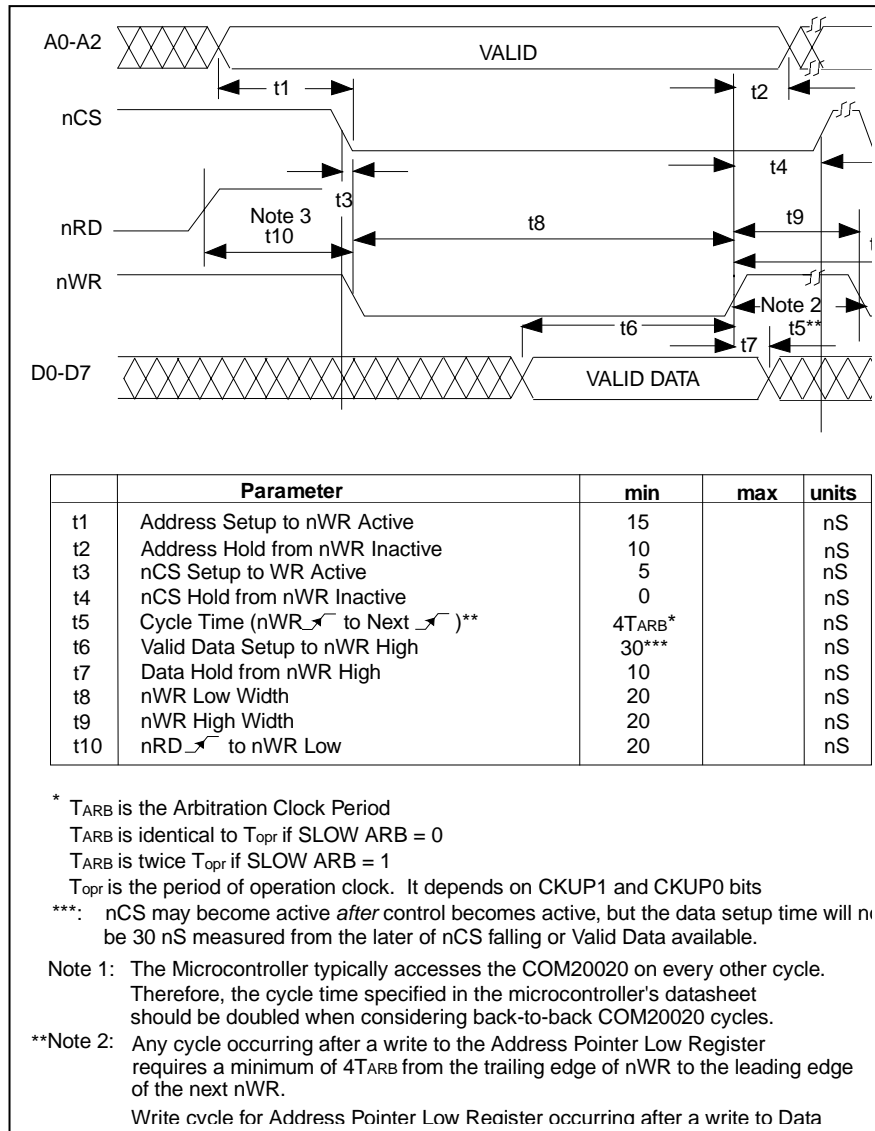
FIGURE 17 - NON-MULTIPLEXED BUS, 80XX-LIKE CONTROL SIGNALS; WRITE CYCLE
