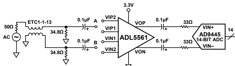
Figure 37. Wideband ADC Interfacing Example Featuring the AD9445
