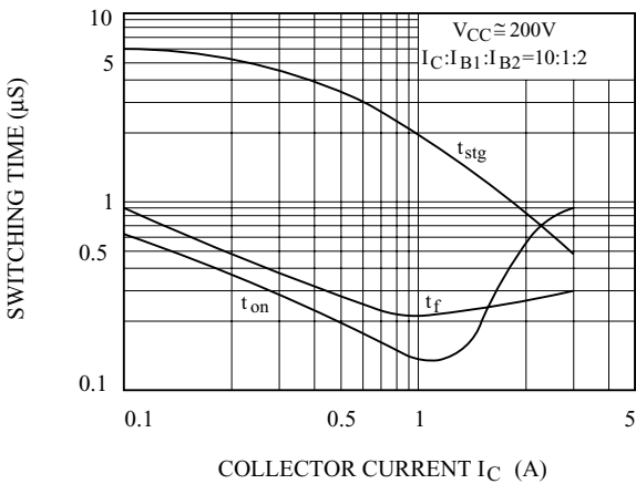
SWITCHING CHARACTERISTICS
