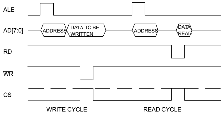
Figure 4. Intel Read and Write Cycles
