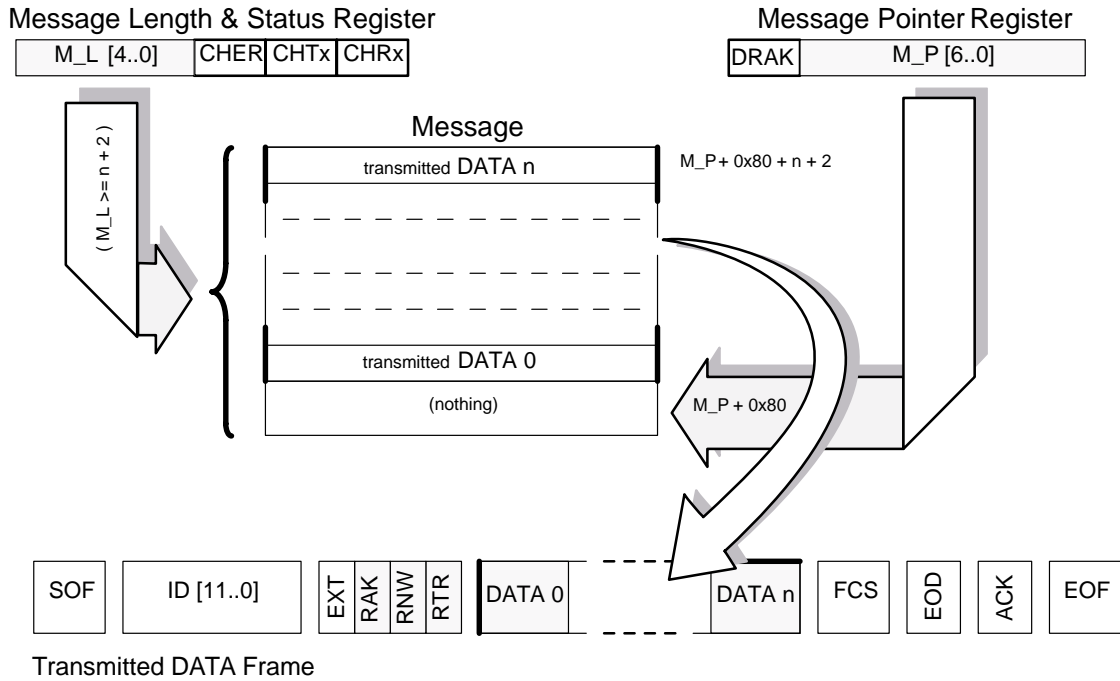
Figure 24. Message Buffer Structure for Transmission
