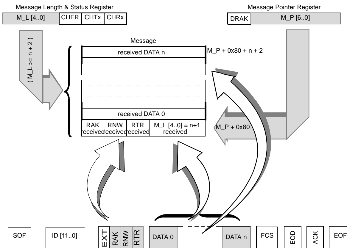
Figure 23. Message Buffer Structure for Reception
