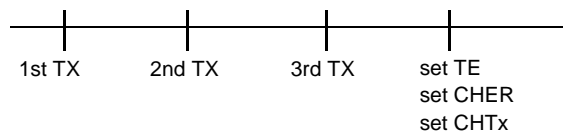
Figure 21. Exceeded retry with MR[3.0] = 3
