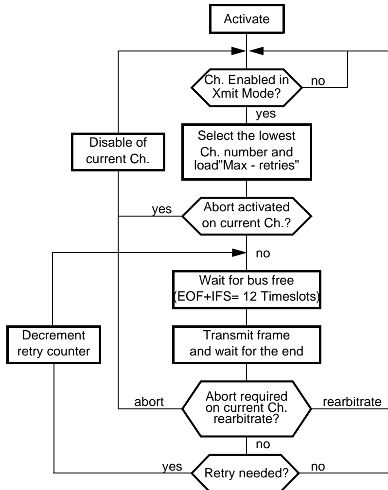
Figure 26. Transmit Function
