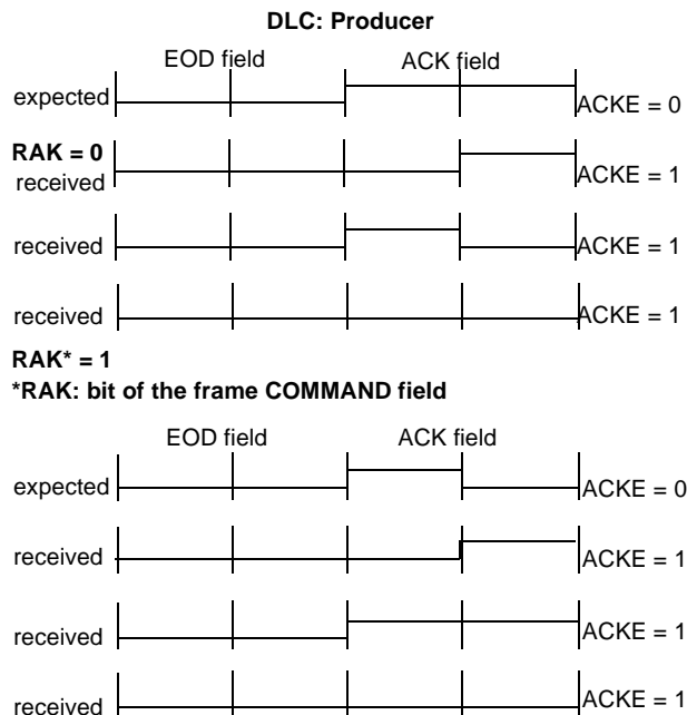
Figure 19. ACKE Status Bit
