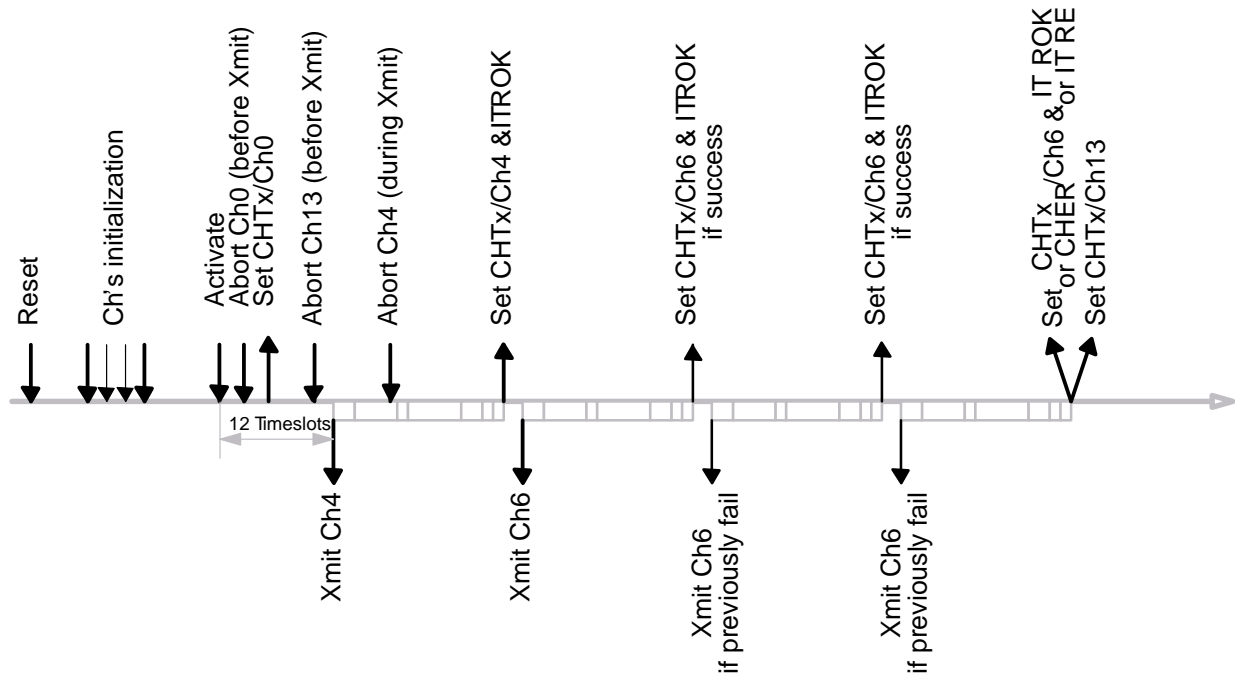
Figure 30. Abort Example
