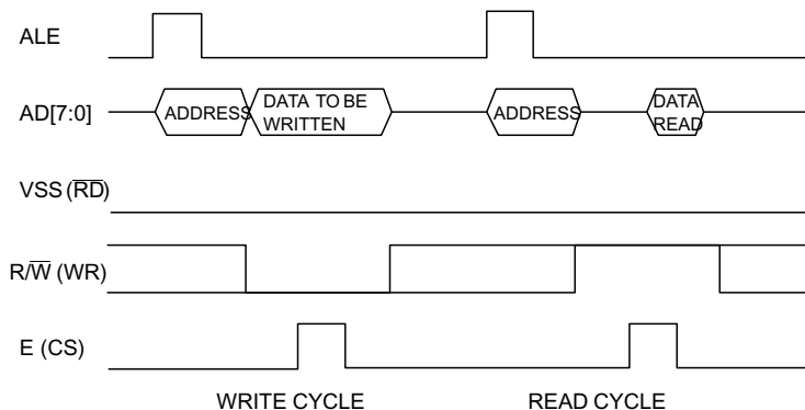
Figure 5. Motorola Read and Write Cycles
