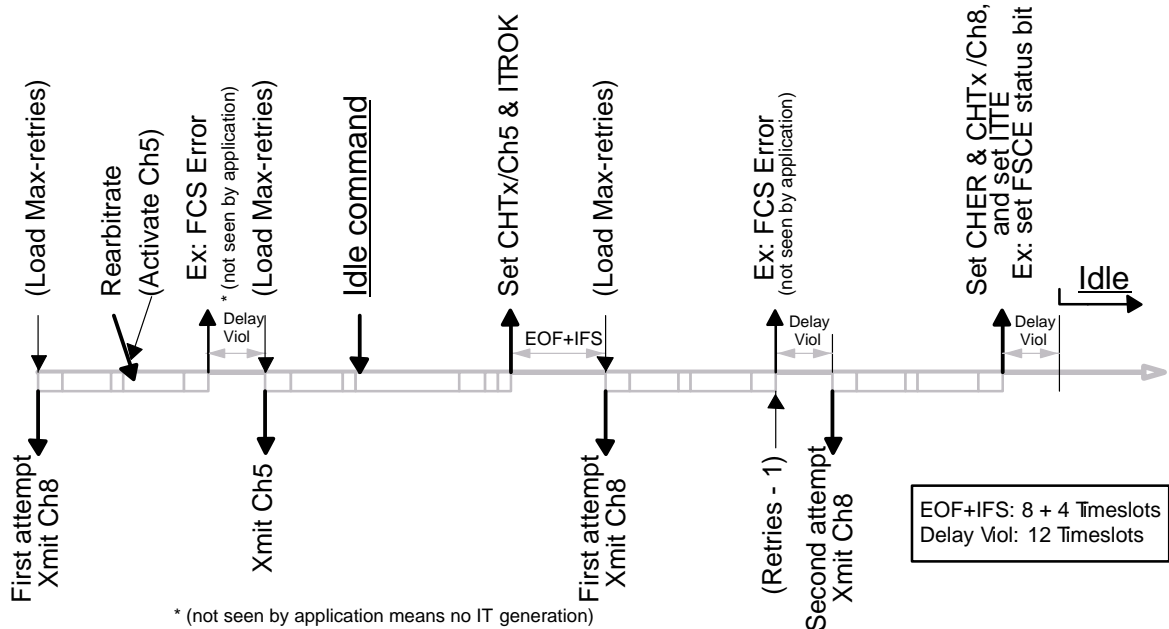
Figure 28. Idle and Rearbitrate Example
