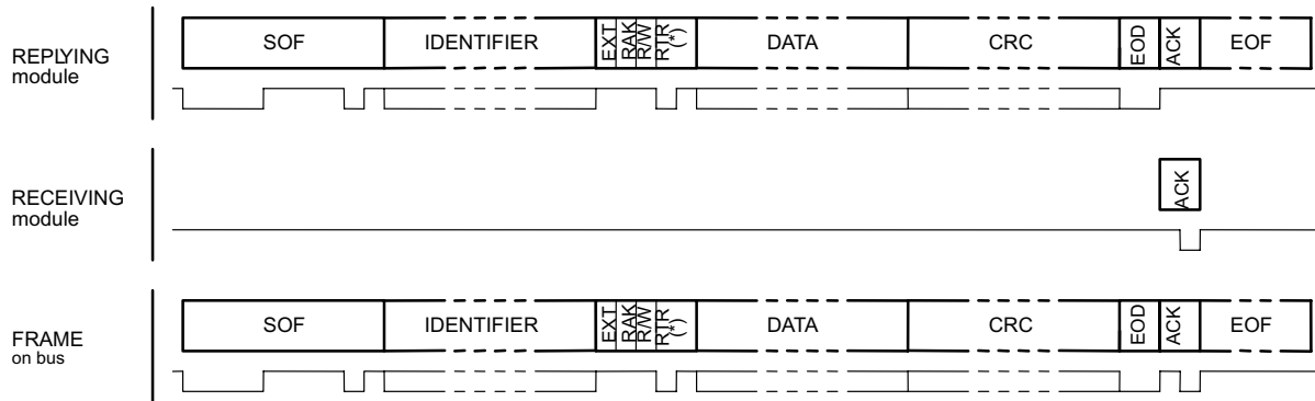
Figure 16. Deferred Reply Frame
