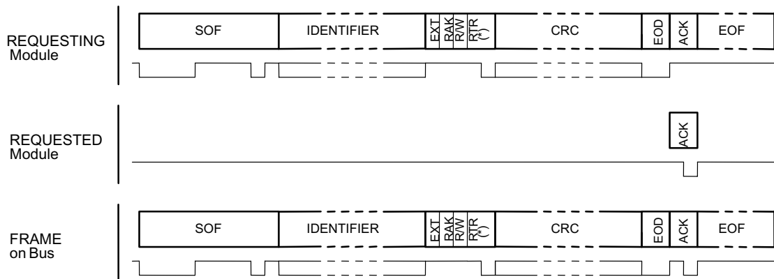
Figure 15. Reply Request Frame with Deferred Reply
