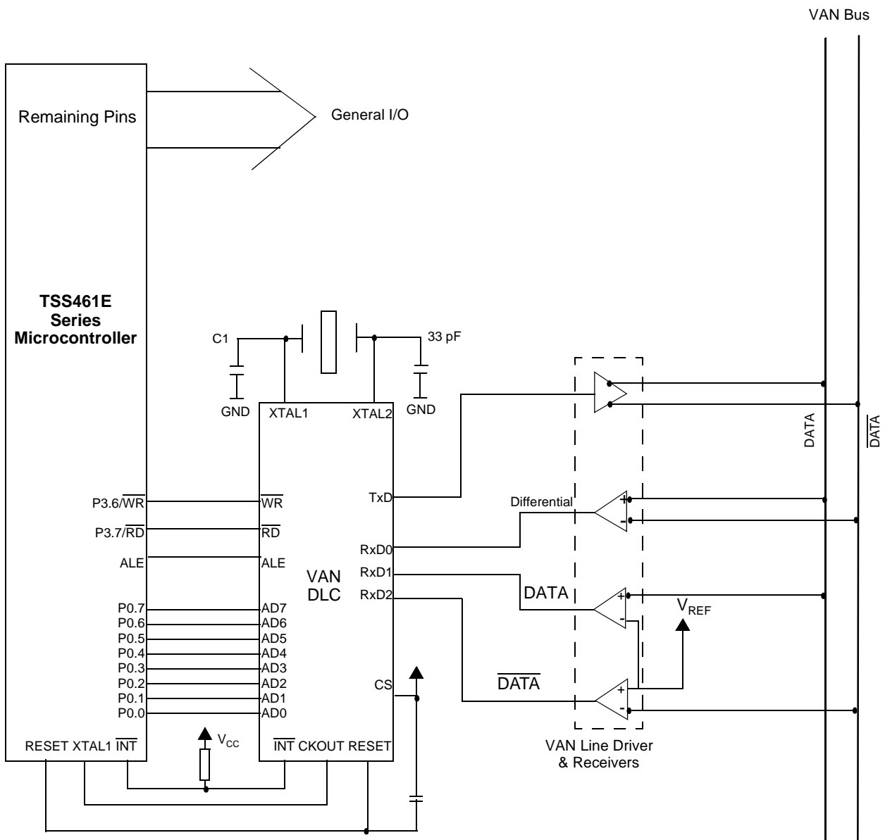
Figure 3. Typical Application
