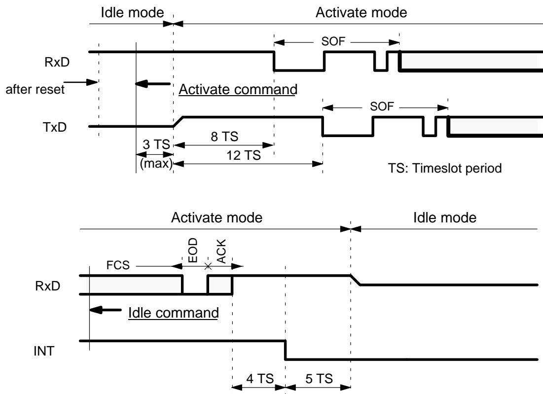
Figure 31. Idle and Activate Timings
