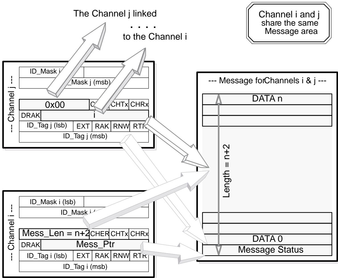
Figure 32. Linkage Mechanism
