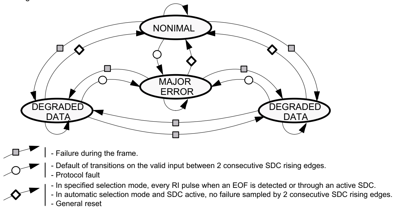
Figure 17. Diagnosis States
