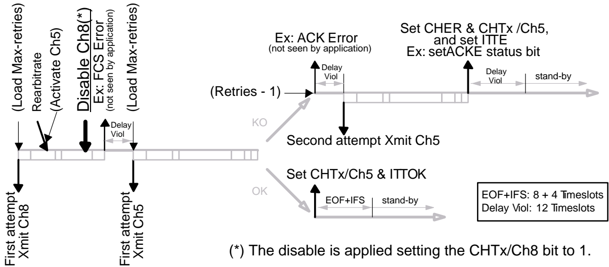
Figure 29. Disable Channel After Rearbitrate Example
