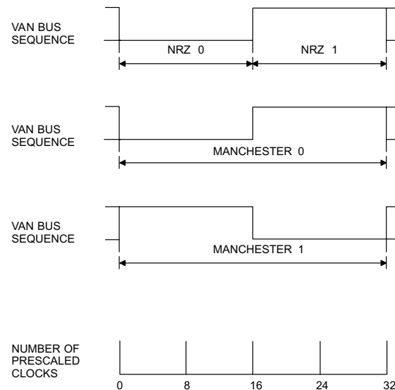
Figure 11. Data Encoding
