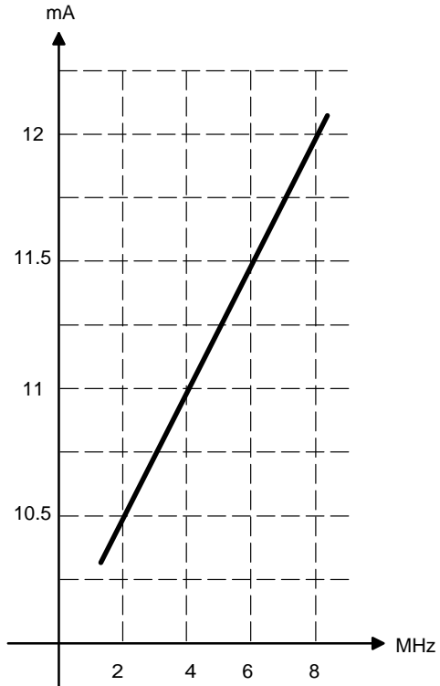
Figure 34. I_{CC} Versus Clock Frequency at 250 KTimeslot/s
