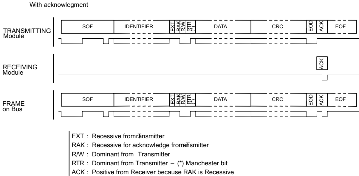
Figure 13. Normal Data Frame
