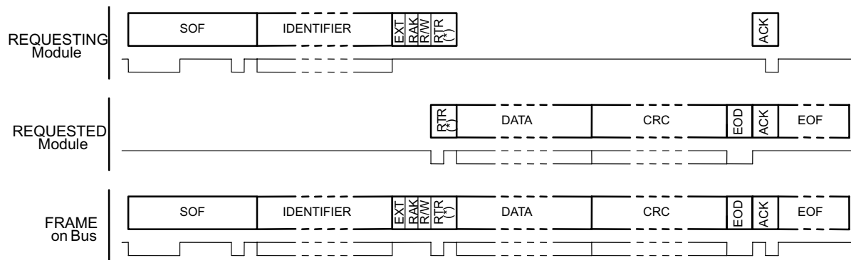
Figure 14. Reply Request Frame with Immediate Reply
