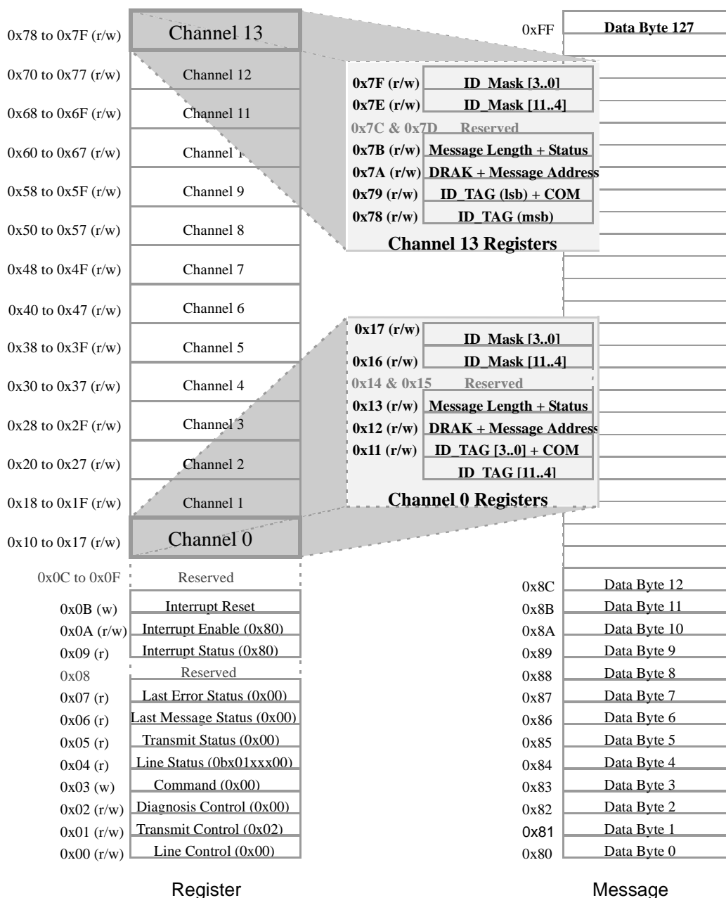
Figure 18. Memory Map
