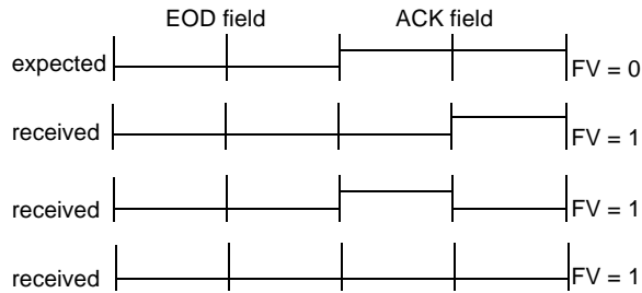
Figure 20. FV Status Bit
