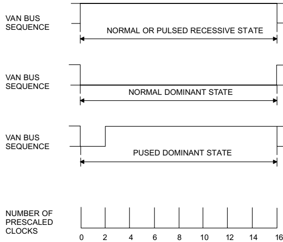
Figure 7. State Encoding
