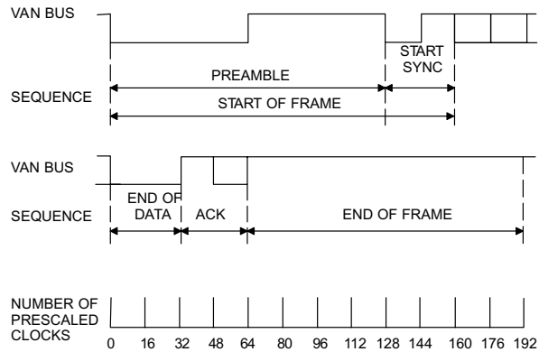
Figure 10. Framing Sequences
