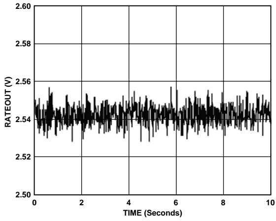
Figure 17. Random Vibration (Lateral) 2 Hz to 40 Hz 3.2 g rms
