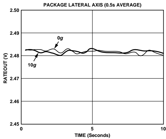
Figure 11. 10 g Random Vibration in Package-Lateral Axis Orientation
