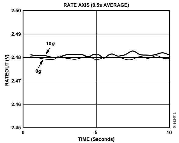
Figure 13. 10 g Random Vibration in Rate Axis Orientation
