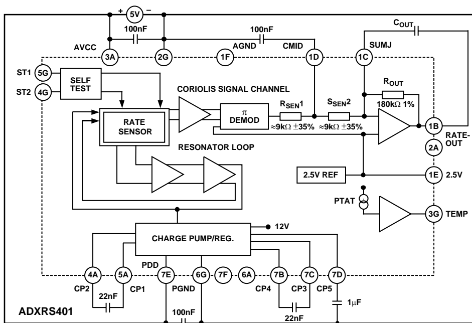
Figure 15. Block Diagram with External Components
