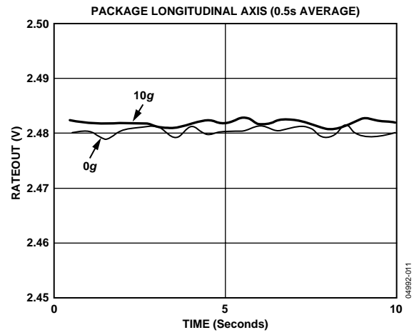
Figure 12. 10 g Random Vibration in Package-Longitudinal Axis Orientation
