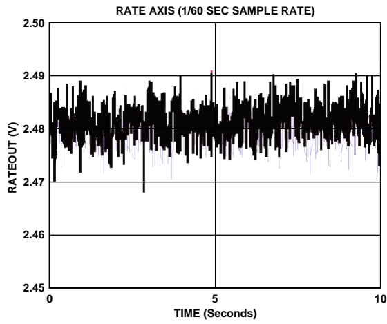
Figure 10. 10 g Random Vibration in Rate Axis Orientation
