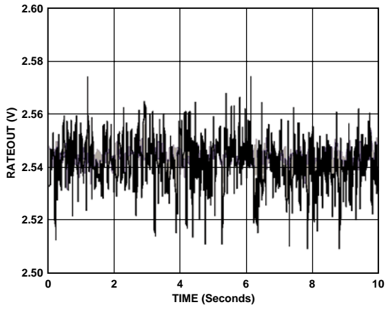
Figure 18. Random Vibration (Lateral) 10 kHz to 20 kHz at 0.01 g/√Hz with 60 Hz Sampling and 0.5 Sec Averaging
