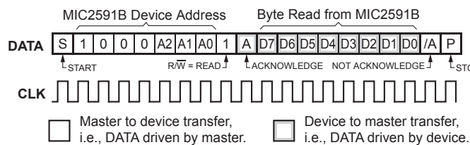
Figure 12. RECEIVE_BYTE Protocol
