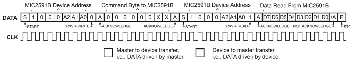
Figure 11. READ_BYTE Protocol
