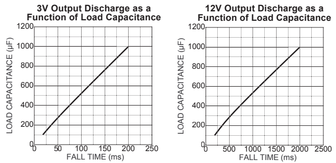
Figure 7. 3V and 12V Output Discharge vs. Load Capacitance
