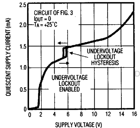
MAX738 QUIESCENT SUPPLY CURRENT vs. SUPPLY VOLTAGE
