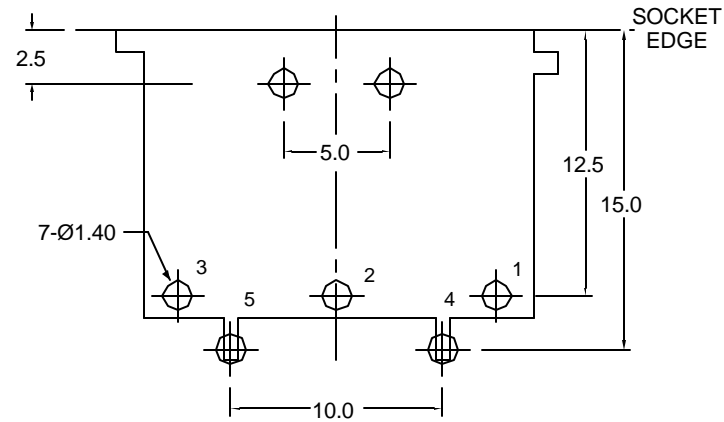
PCB LAYOUT
