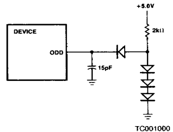
LOAD FOR PARITY OUTPUT
