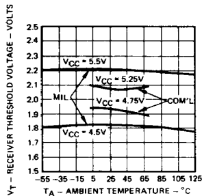
Am2907 Receiver Threshold Variation Versus Ambient Temperature
