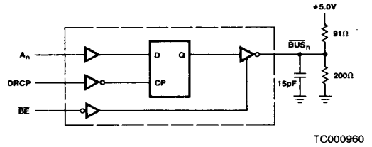
Am2908 DRIVER SWITCHING TEST CIRCUIT
