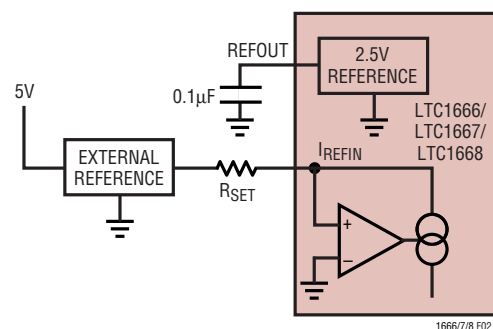
Figure 1. Using the LTC1666/LTC1667/LTC1668 with an External Reference
