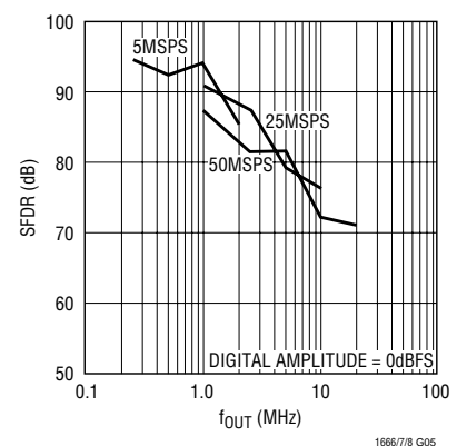
LTC1668 SFDR vs f_{OUT} and f_{CLOCK}
