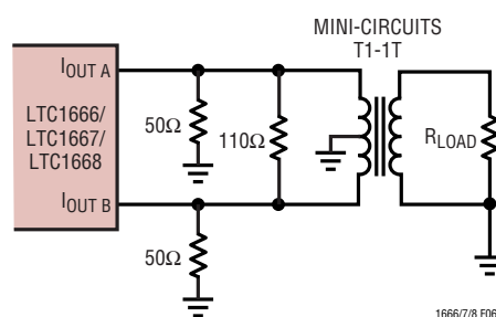
Figure 5. Differential Transformer-Coupled Outputs
