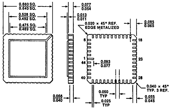
44-Pin Leadless Chip Carrier (LCC), Ceramic, Jeduc Type C
