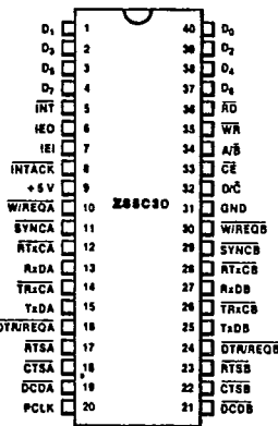
Figure 2a. DIP Pin Assignments, Z85C30
