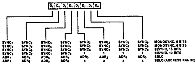
Figure 11. Write Register Bit Functions
