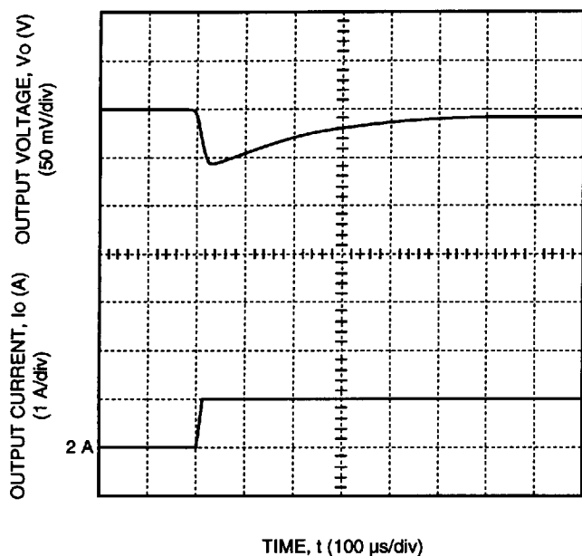
Figure 5. LC020A Typical Output Voltage for a Step Load Change from 50% to 75%
