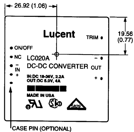
Figure 11. Case Temperature Measurement Location
