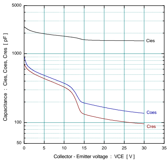
[ Brake ] Capacitance vs. Collector-Emmitter voltage (typ.) V GE =0V, f= 1MHz, T j = 25°C
