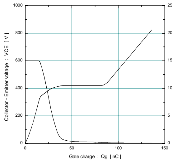
[ Brake ] Dynamic Gate charge (typ.) V CC =600V, I c =15A, T j = 25°C
