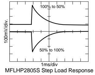
MFLHP2805S Step Load Response
