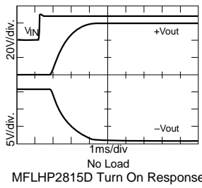
MFLHP2815D Turn On Response
