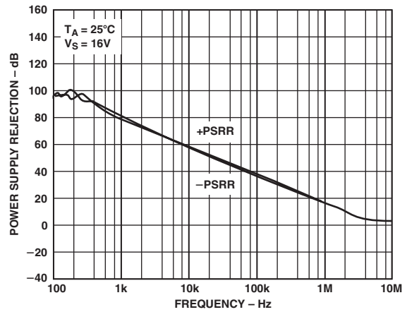
TPC 17. Power Supply Rejection Ratio vs. Frequency
