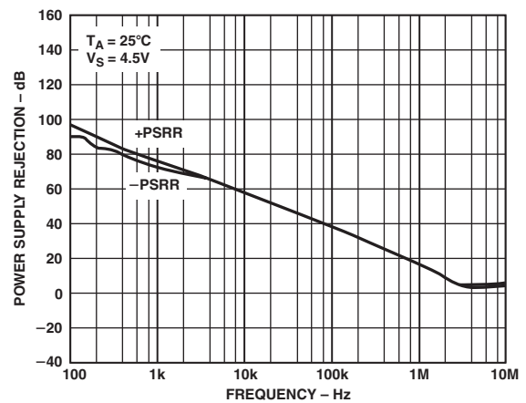
TPC 18. Power Supply Rejection Ratio vs. Frequency
