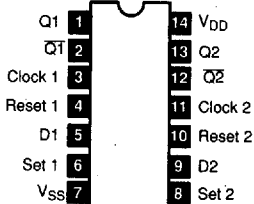
NTE4013B 14-Lead DIP, See Diag. 247 Dual D-Type Flip-Flop
