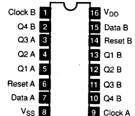
NTE4015B 16-Lead DIP, See Diag. 249 Dual 4-Stage Static Shift Register w/Serail Input/Parallel Output
