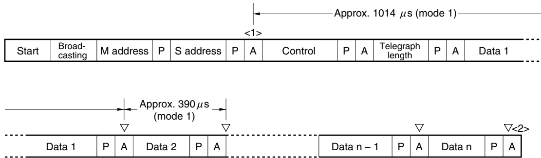
Figure 18-20. Slave Reception
