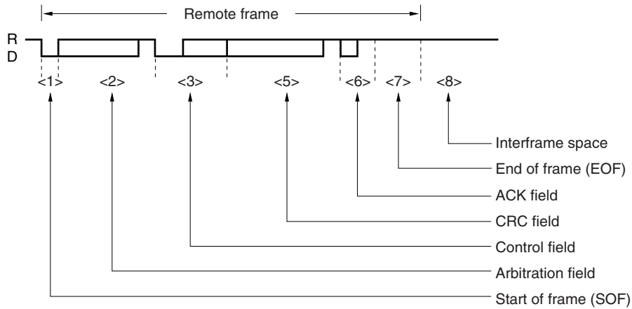
Figure 19-12. Remote Frame
