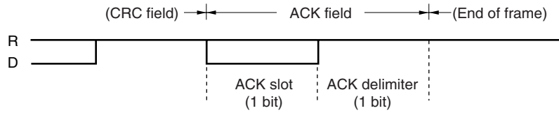
Figure 19-19. ACK Field
