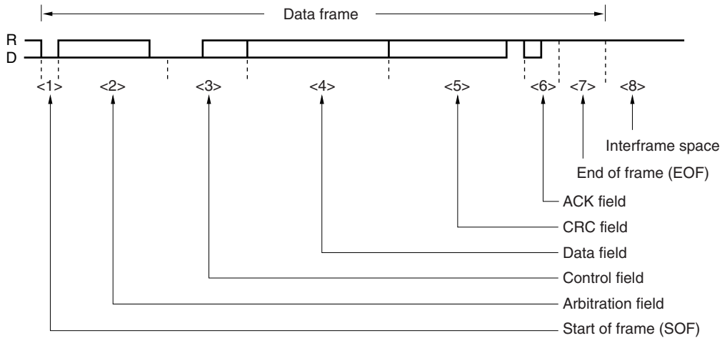
Figure 19-11. Data Frame
