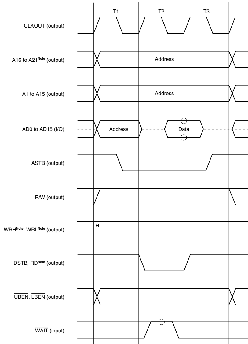
Figure 6-8. Memory Read (1/4)
