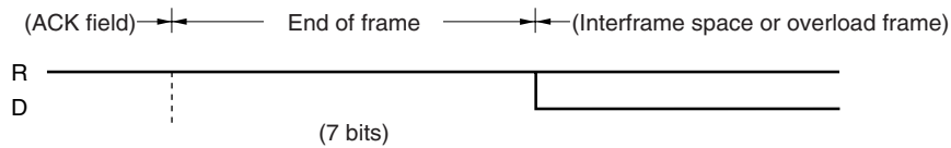
Figure 19-20. End of Frame (EOF)
